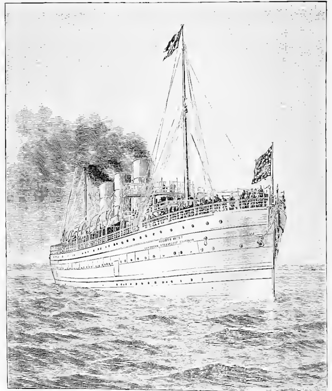
THE TWIN-SCREW STEAMERS NORTH WEST AND NORTH LAND.—Built by the Globe Iron Works, Cleveland, Ohio.
